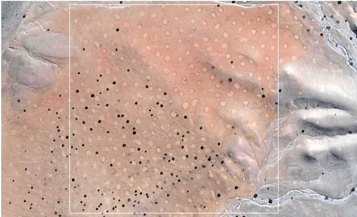
Fig. S2 Google satellite image from 2016 of the plot Gir-1, where Theron [6] marked the Euphorbias, fairy circles and control locations in the matrix. The white square shows the 500 m \times 500 m extent of the drone-mapped plot. As the image shows, there are numerous FCs and Euphorbia damarana to enable statistical comparisons between the two types of objects, including spatially-explicit analysis of the patterns with the g - and L -functions. Note the large sizes of the FCs while Euphorbias are comparatively small.
