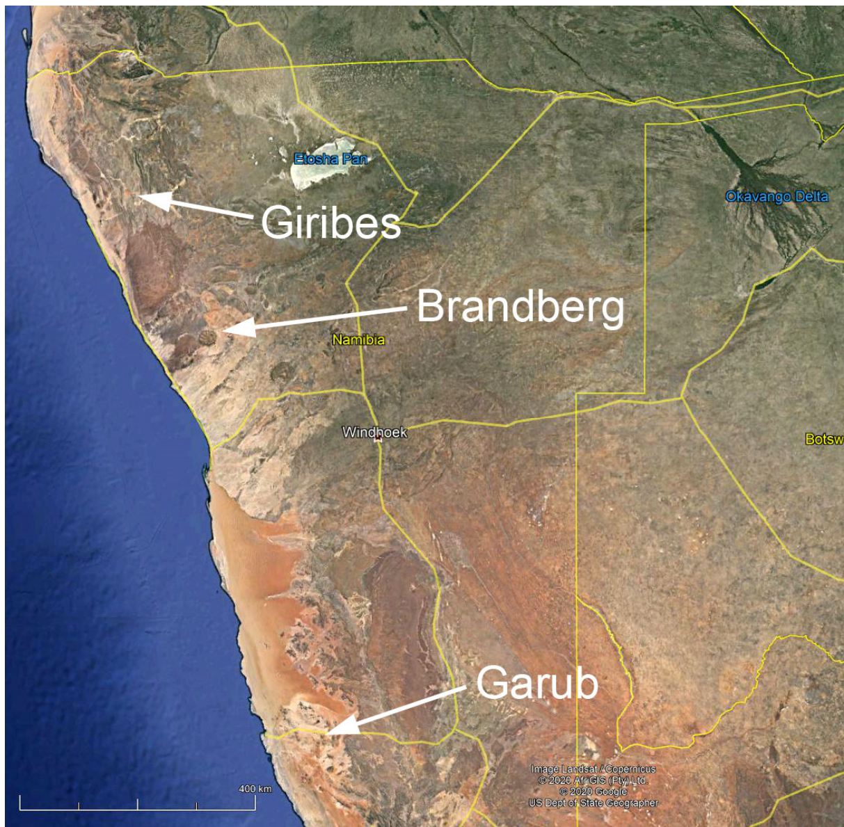
Fig. S1 Google satellite image showing the three study regions Giribes and Brandberg (with Euphorbia damarana ) and Garub (with E. gummifera ).
