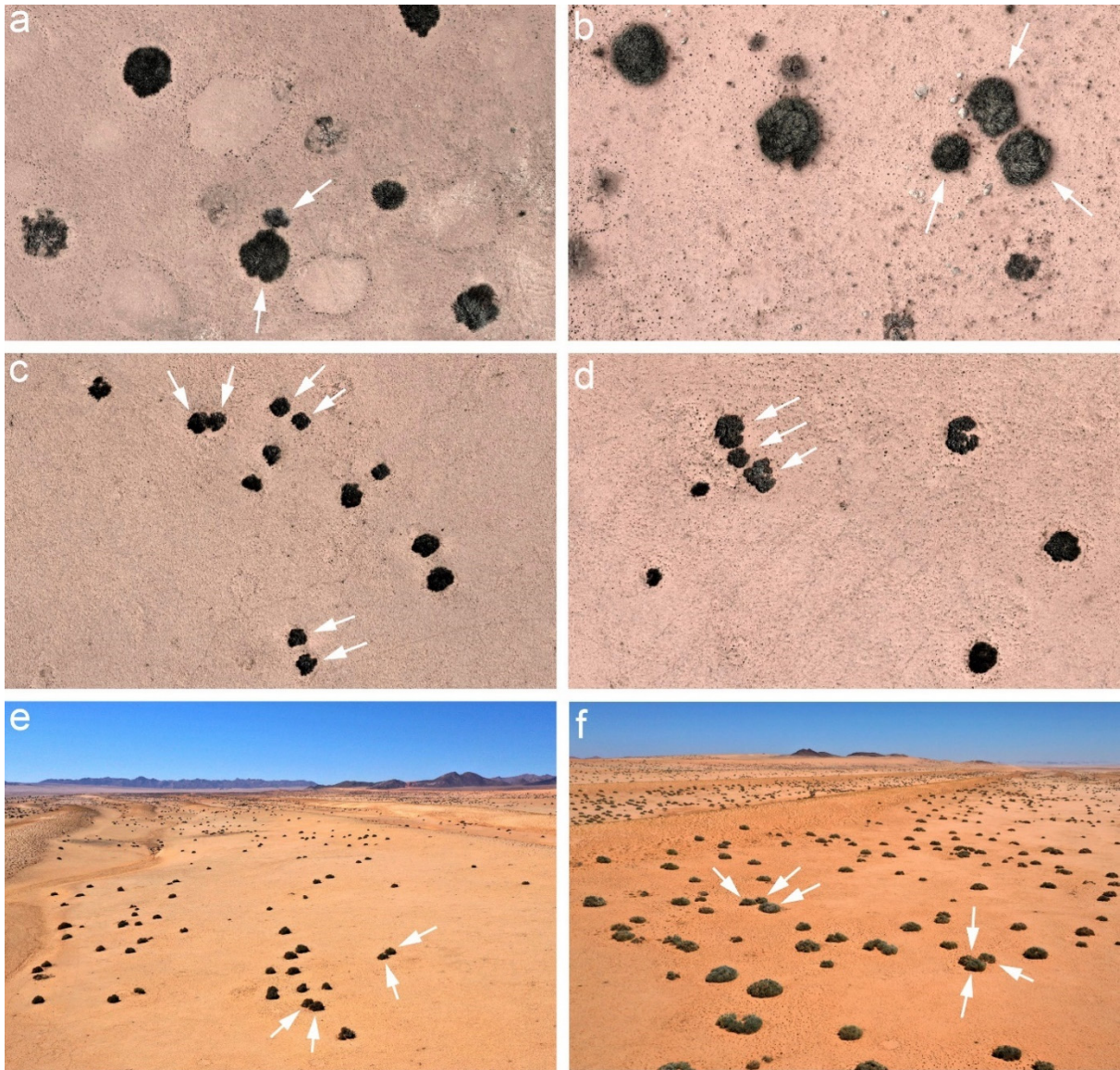
Fig. S7 Evidence for clustered patterns of E. damarana and E. gummifera . Euphorbia damarana in the Theron-plot Gir-1 of the southern Giribes (a) and in the plot Bra-2 near Brandberg (b) showed statistically significant clustering because regeneration of the shrubs often happens in a clumped distribution where individual shrubs are tightly packed together (arrows). Also, Euphorbia gummifera in the plot Gar-1 near Garub showed strongly clustered patterns (c) while in the plot Gar-2 the Euphorbias showed a mixed pattern of clustered and random distributions (d). The clustering results from individual shrubs growing next to each other (arrows) as the high-resolution ortho-images from drone mapping demonstrate. Such a pattern is in contrast to the distribution of FCs because in many FC areas such as the Giribes, the Brandberg, Marienfluss Valley or the NamibRand Nature Reserve, FCs have typically no neighbors in their immediate neighborhood. Also, oblique drone images with overviews over the plots Gar-1 (e) and Gar-2 (f) near Garub clearly show how the individual shrubs with their humped growth form are tightly clustering but they do not have a regularly spaced pattern.
