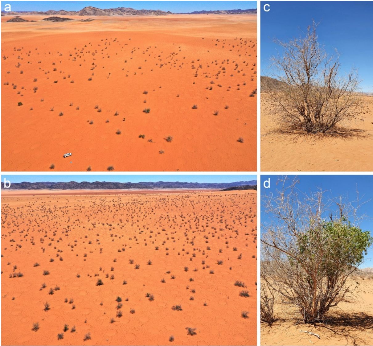
Fig. S8 In the north-eastern part of the Giribes Plains, the species Parkinsonia africana co-occurs in various densities with fairy circles over an area of several square kilometers. Two examples have been photographed in March 2020 with a drone (a,b). Parkinsonia africana is a shrub species or small tree, which may grow on its own (c) or it may be occupied by Salvadora persica which scrambles into it (d).
