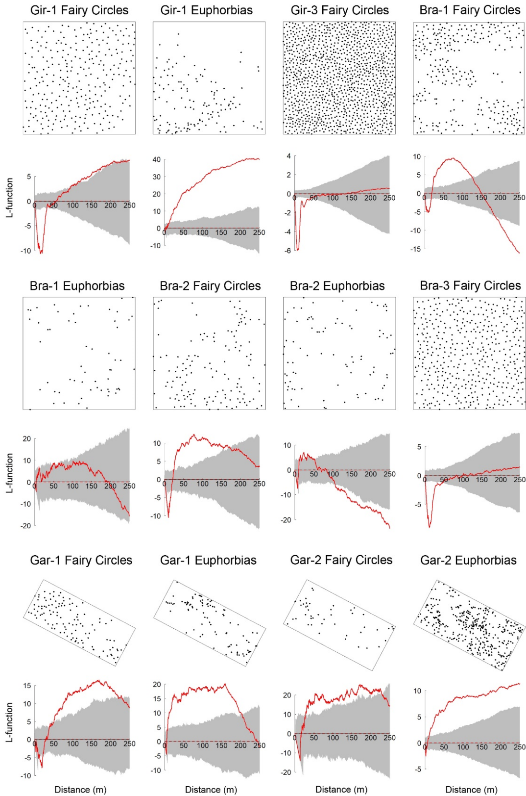
Fig. S3 The large-scale spatial distributions of fairy circles and Euphorbias, assessed with the L -function. The pattern is regular or aggregated at circular neighborhood distances if the red line of the L -function is below the lower or above the upper grey lines of the simulation envelopes, respectively. Null model envelopes were constructed using the 5th-lowest and 5th-highest value of 199 Monte Carlo simulations of the randomly distributed Poisson point process (CSR). The mapped point patterns of the FCs and Euphorbias are shown above the L -functions for the Giribes (Gir-1, Gir-3), the Brandberg (Bra-1, Bra-2, Bra-3) and Garub (Gar-1, Gar-2).
