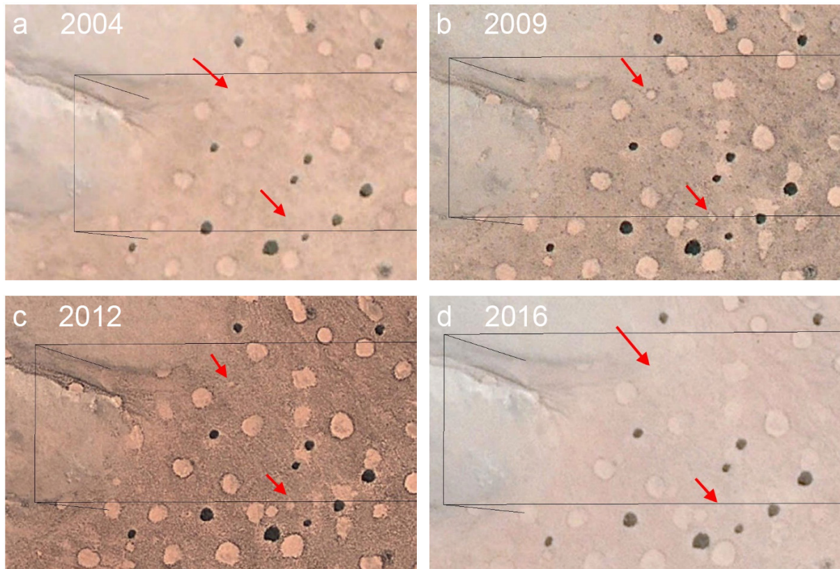
Fig. S4 Formation of new FCs in the Theron-Plot Gir-1. The four Google-Earth satellite images from 2004 to 2016 show how FCs emerge at places where there was no Euphorbia before (a-d). The arrows in the image from 2009 point to two examples of new FCs (b), while there was no Euphorbia at that location in 2004 (a). Large, established FCs are long-lived structures with lifespans reaching at least half a century. However, new born FCs may disappear again (d), which is mainly attributed to cycles of rainfall variation.
