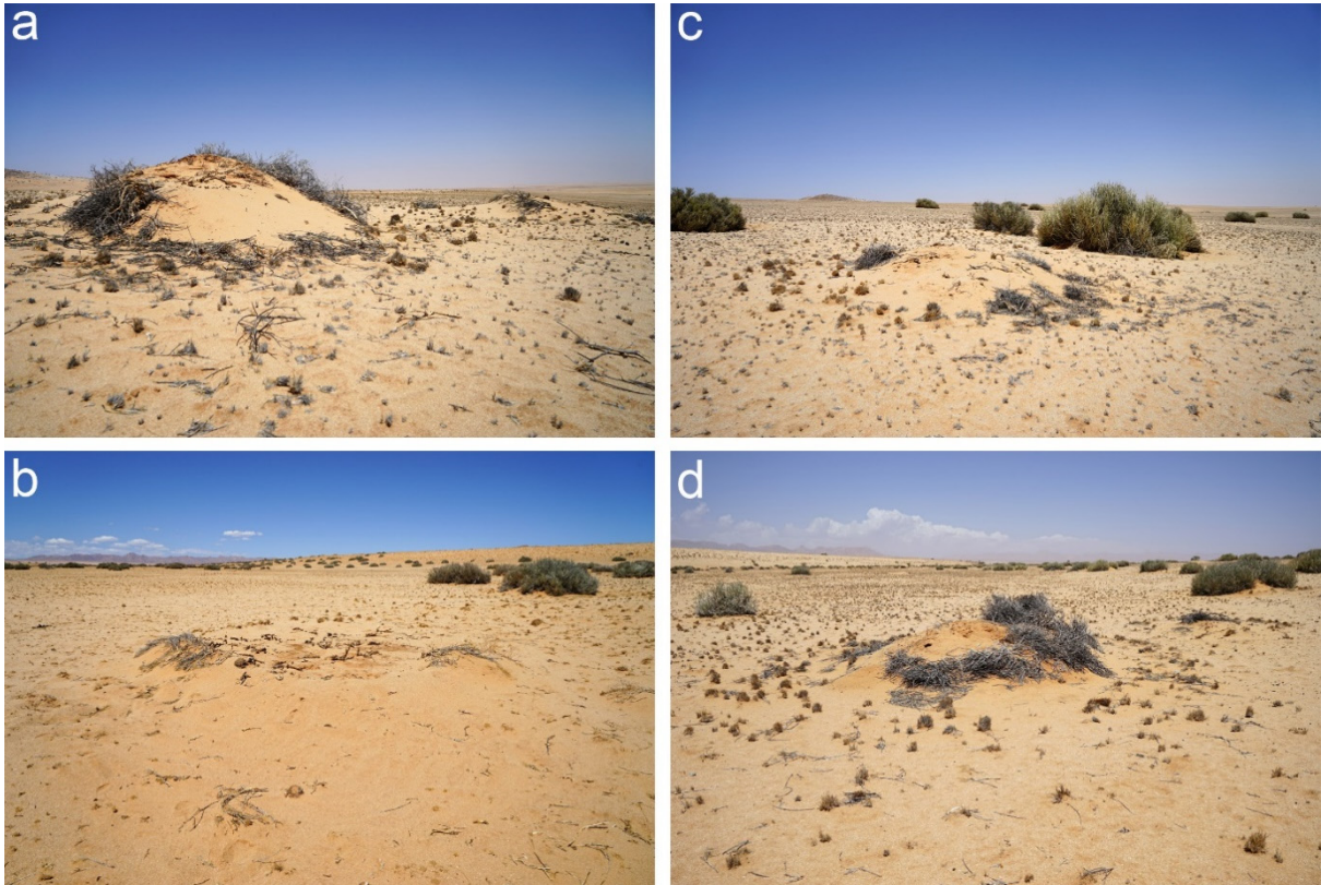
Fig. S6 Several examples of typical sand piles, accumulating around decaying Euphorbia gummifera at the two sites Gar-1 and Gar-2 near Garub (a-d). These circular sand piles with reduced vegetation cover may look similar to fairy circles in aerial or satellite imagery. However, these piles of sand cannot be called fairy circles.
